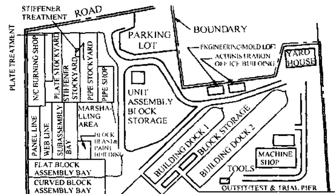
Fig. 19.2 Representative shipyard layout
