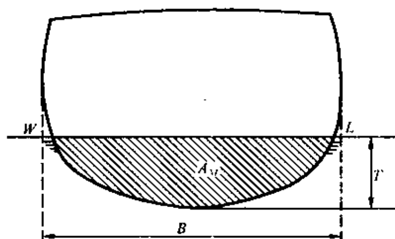
Figure 4.10 Midship coefficient
