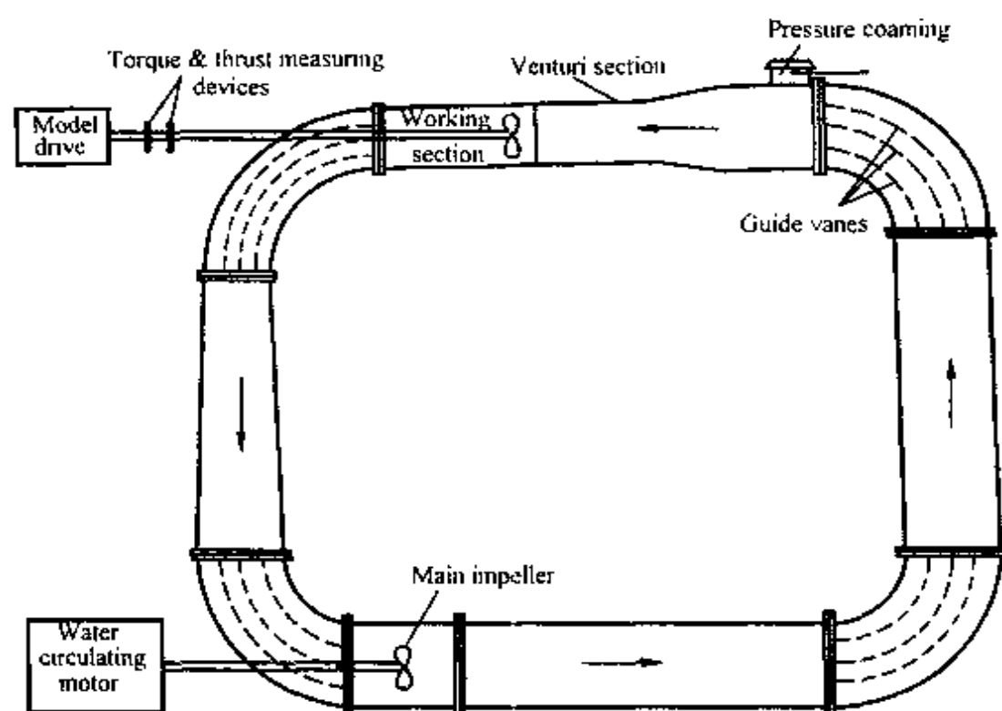
Fig. 11.4 Diagrammatic arrangement of a cavitation tunnel
