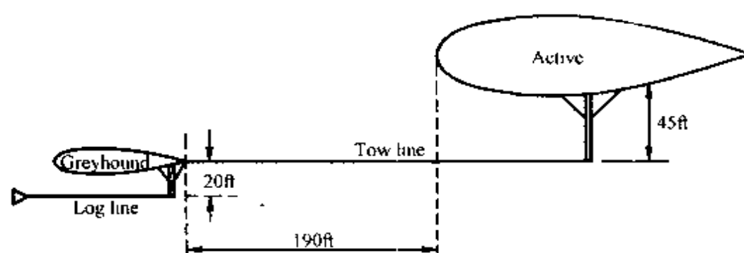
Fig. 11.7 Greyhound experiments
