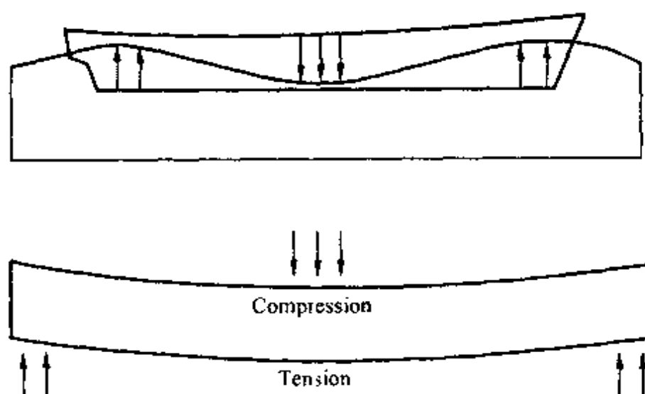
Fig. 14.1 Sagging condition
