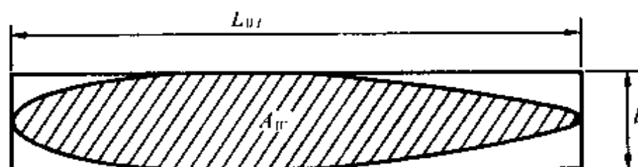
Figure 4.9 Waterplane coefficient
