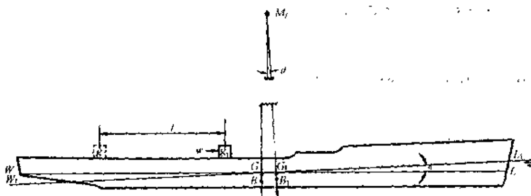
Figure 7.4 Longitudinal stability
