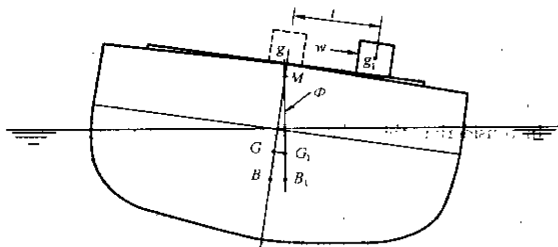
Figure 7.3 Inclined equilibrium
