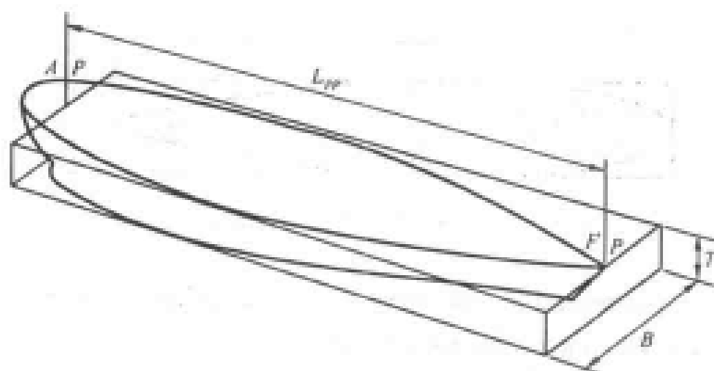
Figure 4.11 Block coefficient
